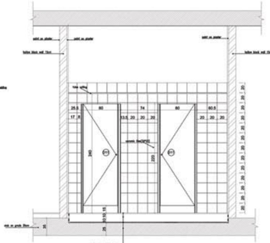
section-1- scale:1/20
