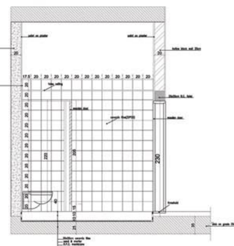
section-1- scale:1/20
